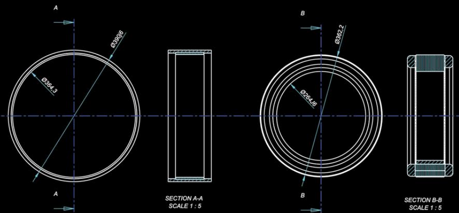
EXTERNAL ROTOR
